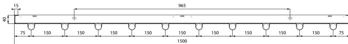
DS-ST28-2-150; 10 Pipes
