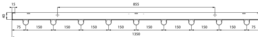
DS-ST28-2-150; 10 Pipes
