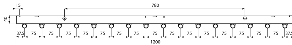
DS-ST18-4-120; 16 Pipes
